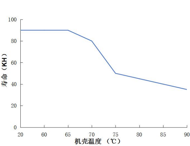
Tc VS 寿命(HVE-100H-38/56/143A/B)
