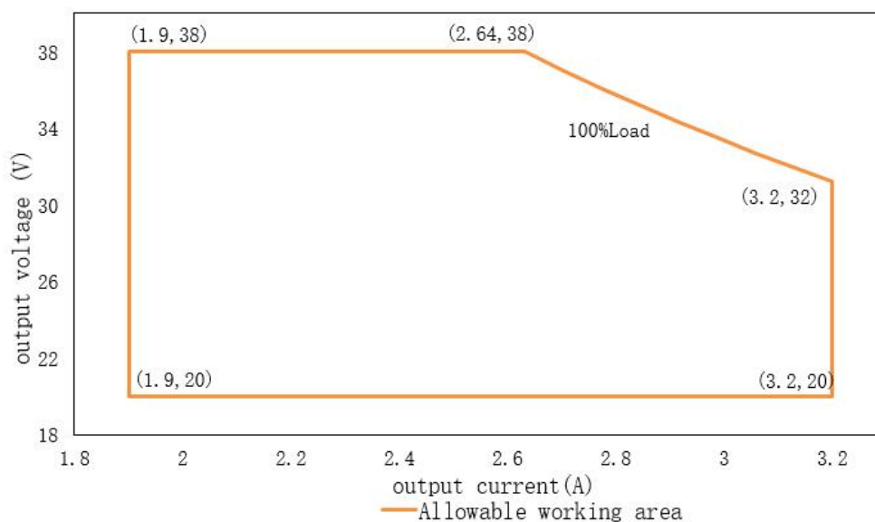
HVE-100H-38A/B (input:200-277Vac) output voltage VS Output current
