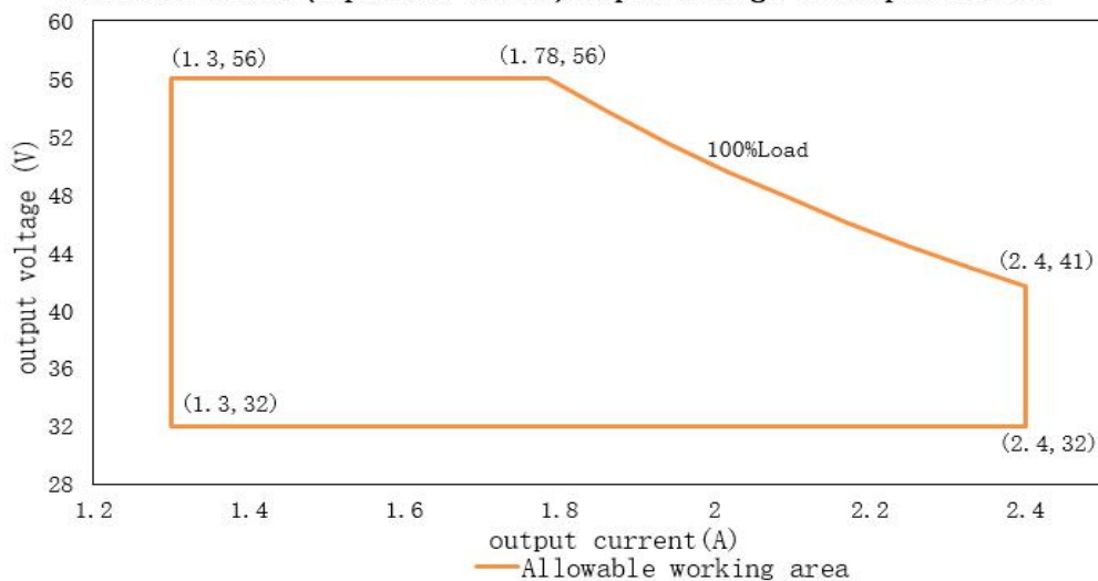
HVE-100H-56A/B (input:200-277Vac) output voltage VS Output current
