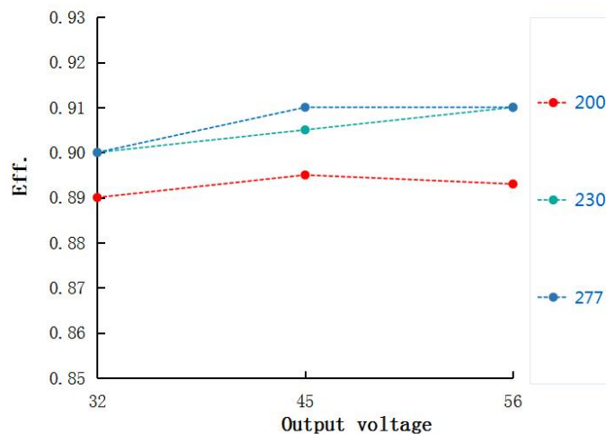
Eff. VS Output voltage HVE-100H-56A/B
