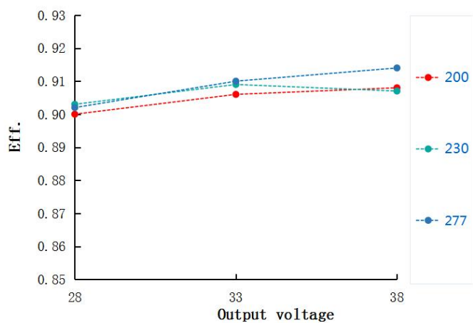
Eff. VS Output voltage HVE-100H-38A/B
