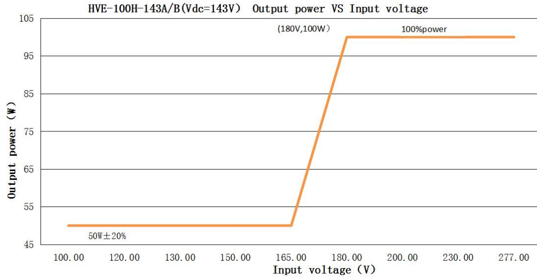
HVE-100H-143A/B(For output 143Vdc, the rated output current & power under different input voltage)
