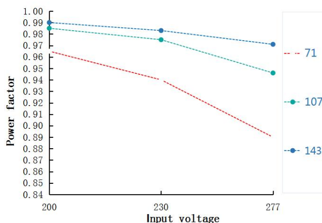
Power factor VS Input voltage HVE-100H-143A/B
