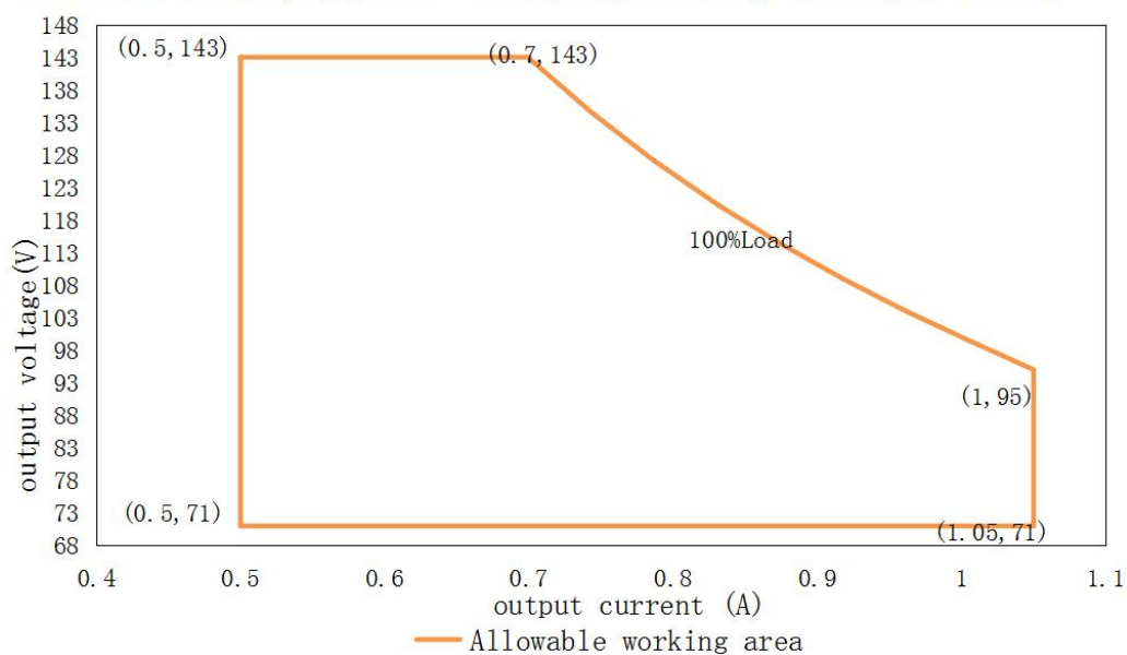
HVE-100H-143A/B (Import:200-277Vac) output voltage VS output current
