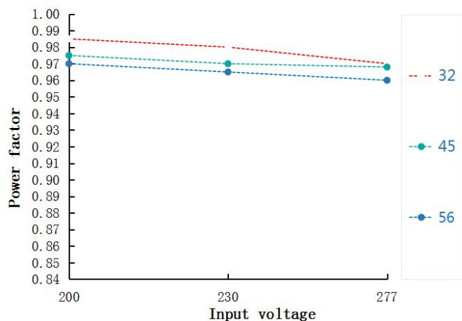
Power factor VS Input voltage HVE-100H-56A/B
