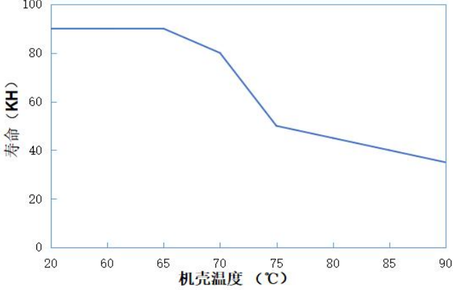
Tc VS 寿命 ( HAE-12W )
