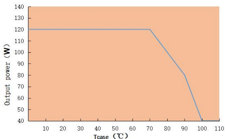
Output power VS Tcse
