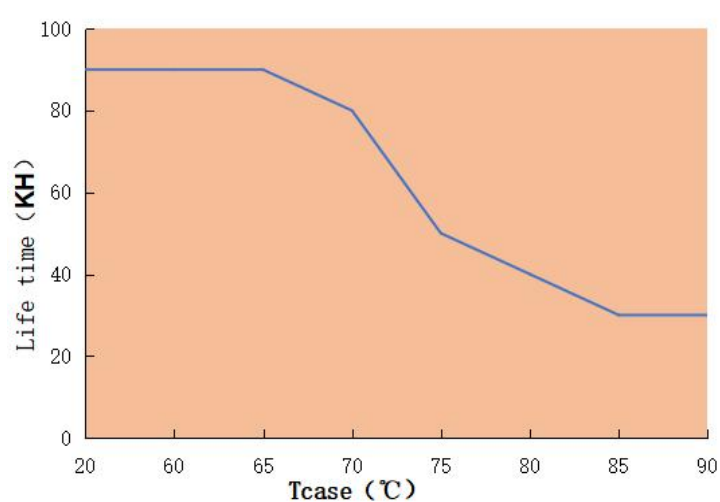
Tcse VS Life time
