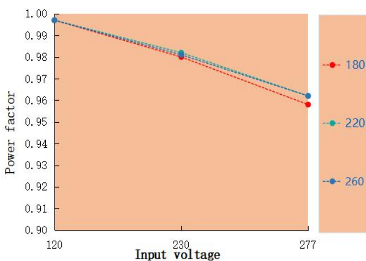
Power factor VS Input voltage
