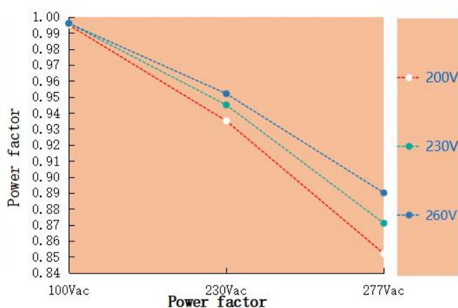
Power factor VS Input voltage
