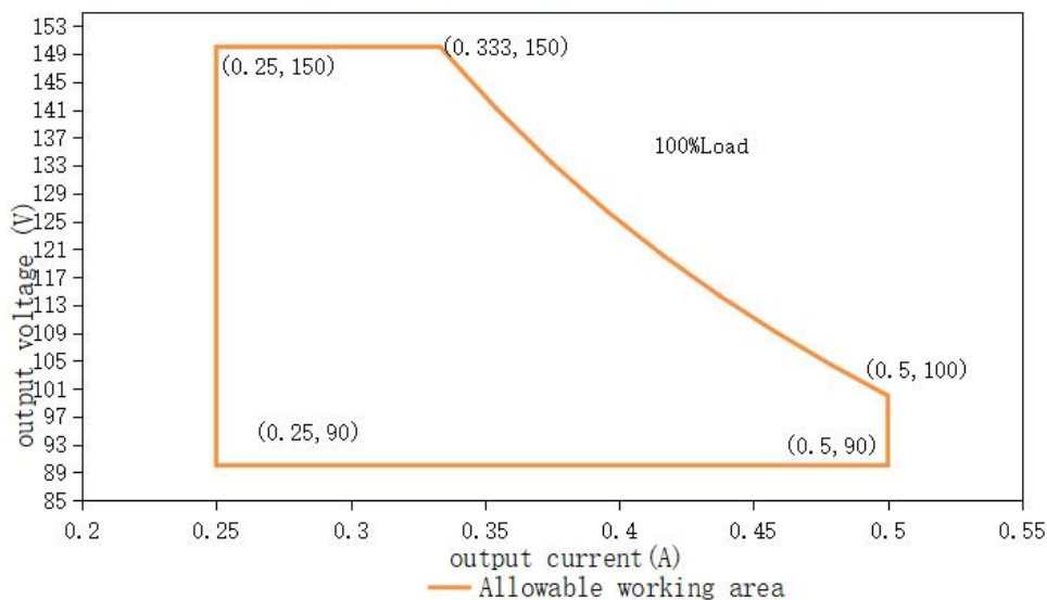
HVS-50W-150X(input:100-277Vac)output voltage VS Output current
