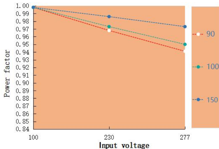
Power factor VS Input voltage
