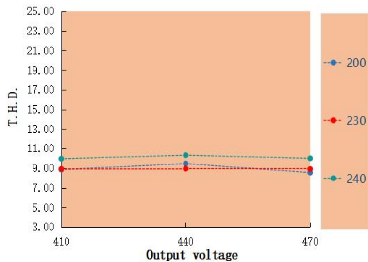
T.H.D. VS Output voltage LAS-150H-470A-XP
