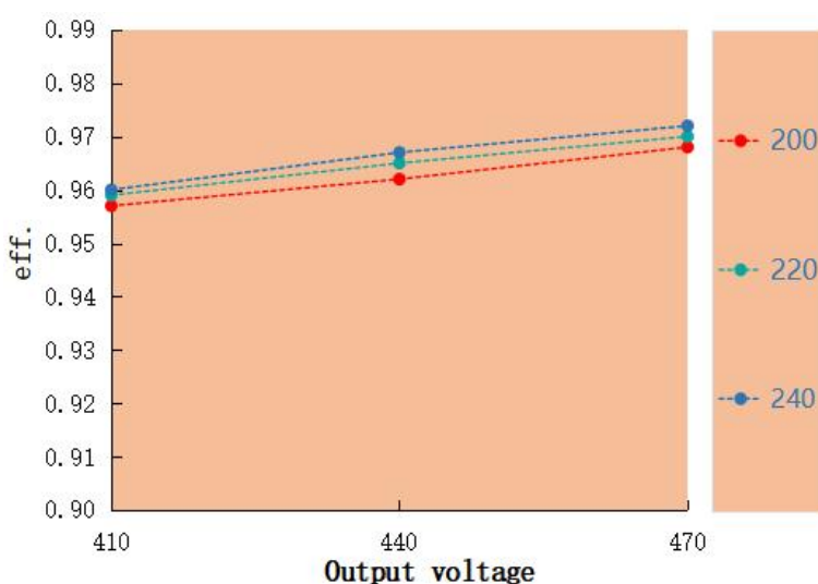
Eff. VS Output voltage LAS-150H-470A-XP
