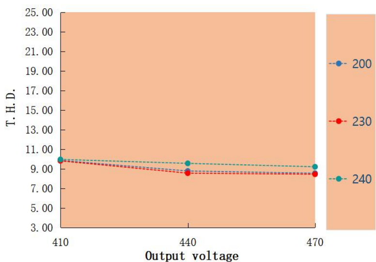
T.H.D. VS Output voltage LAS-150H-470A
