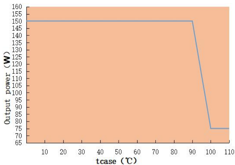
Output power VS Tcase LAS-150H-470A
