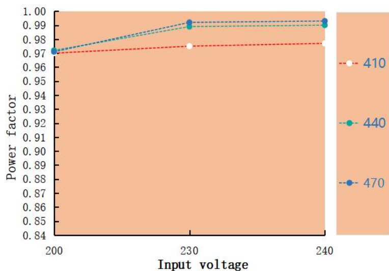
Power factor VS Input voltage LAS-150H-470A
