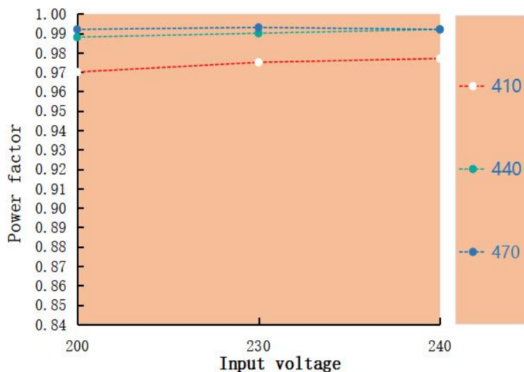
Power factor VS Input voltage LAS-150H-470A-XP
