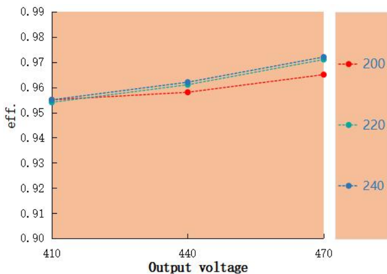
Eff. VS Output voltage LAS-150H-470A
