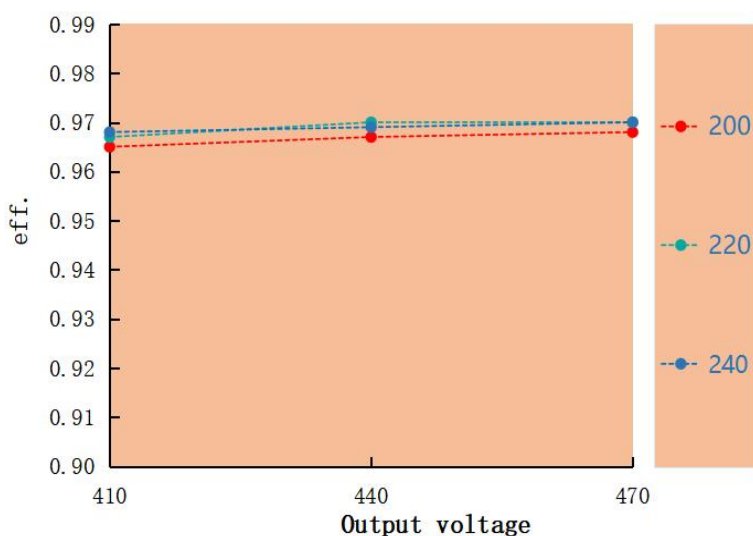
Eff. VS Output voltage LAS-100H-470A
