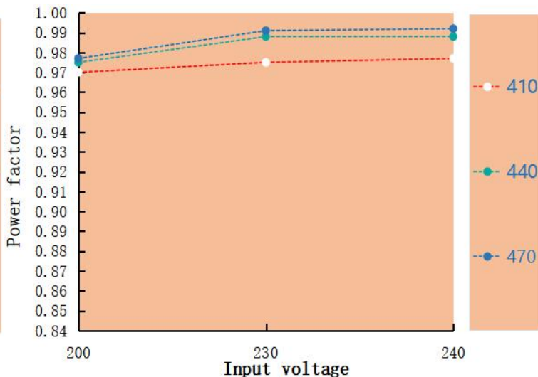
Power factor VS Input voltage LAS-100H-470A-XP
