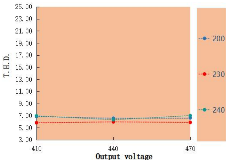
T.H.D. VS Output voltage LAS-100H-470A
