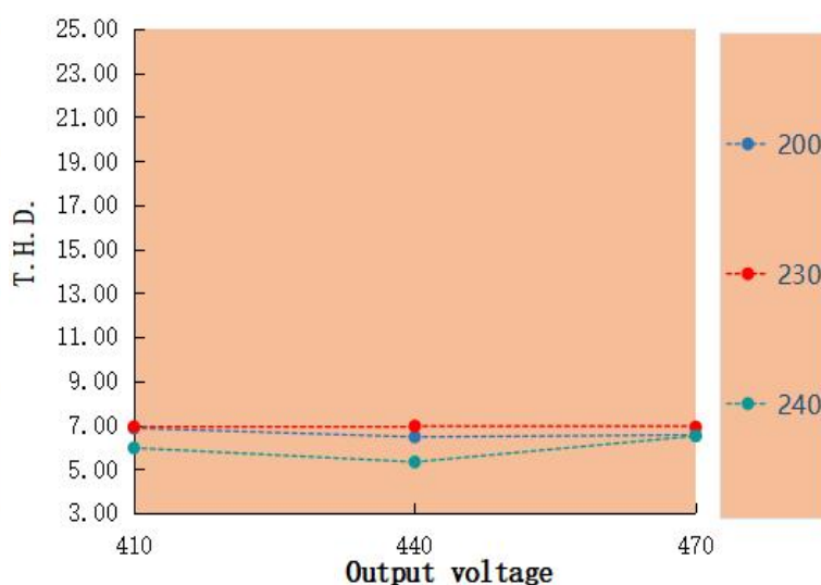
T.H.D. VS Output voltage LAS-100H-470A-XP
