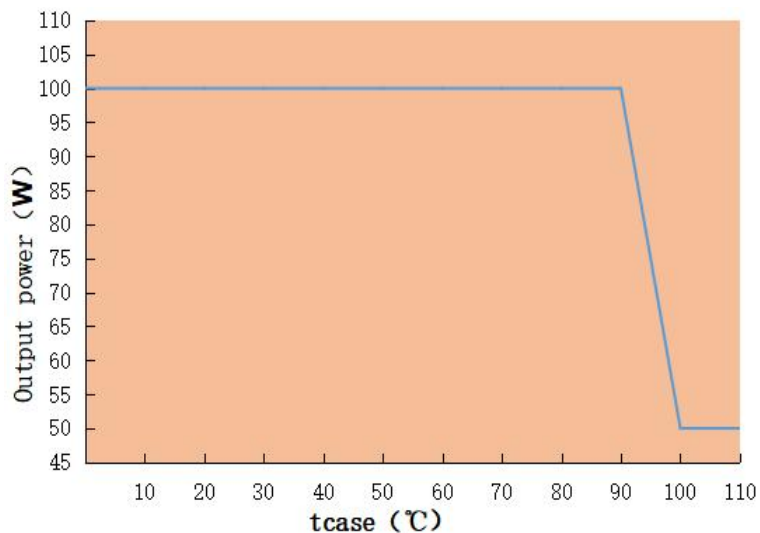
Output power VS Tcase LAS-100H-470A
