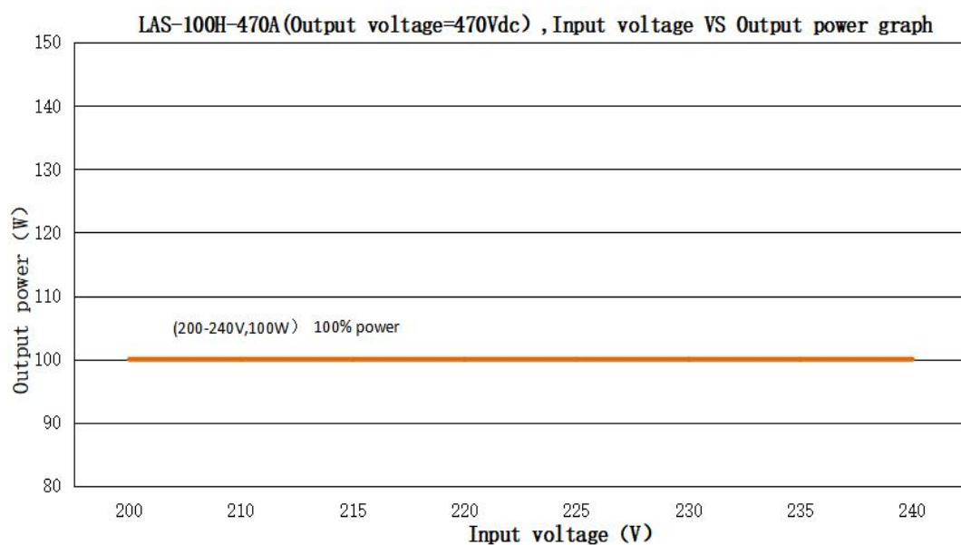
LAS-100H-470A(Vdc=470Vdc, the rated output current & power under different input voltage)
