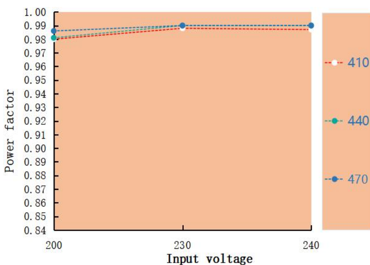
Power factor VS Input voltage LAS-100H-470A
