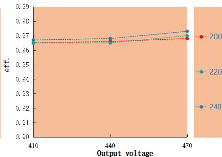
Eff. VS Output voltage LAS-100H-470A-XP
