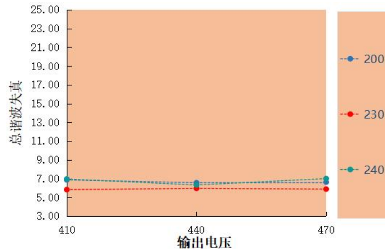
总谐波失真 VS 输出电压 LAS-100H-470A
