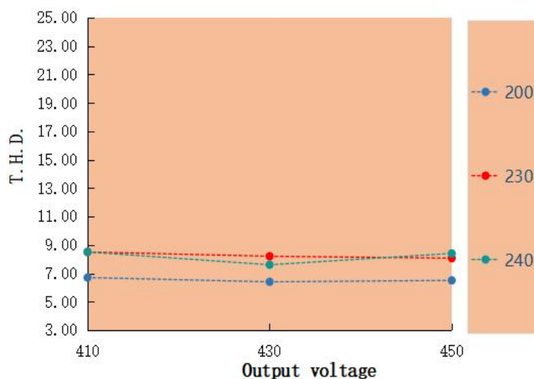
T.H.D. VS Output voltage LAG-200H-450A-XP
