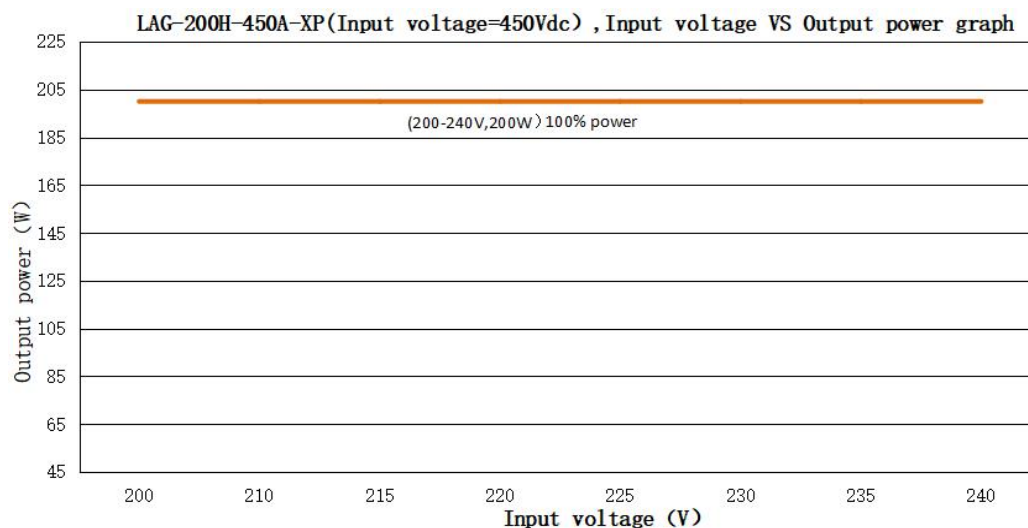
LAG-200H-450A-XP (Vdc=450Vdc, the rated output current & power under different input voltage)
