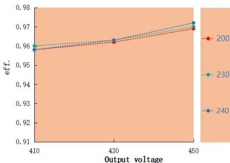
Eff. VS Output voltage LAG-200H-450A-XP
