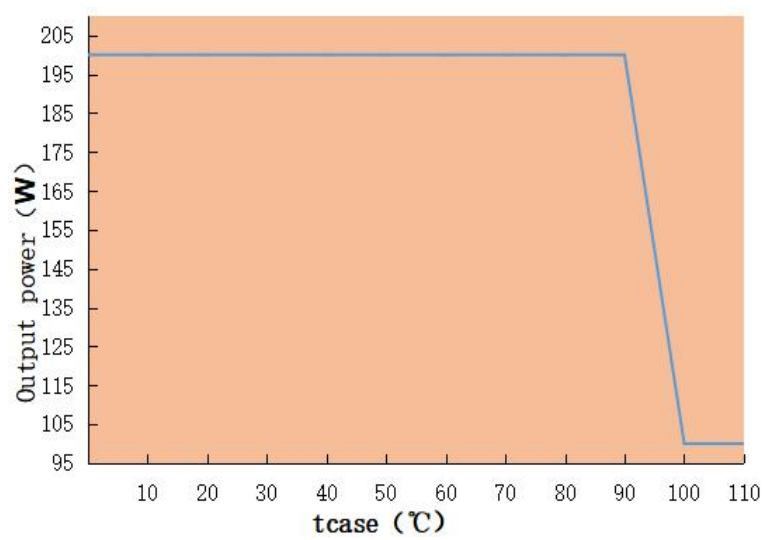
Output power VS Tcase LAG-200H-450A
