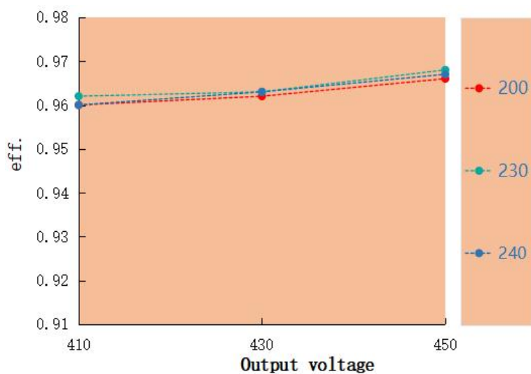
Eff. VS Output voltage LAG-200H-450A
