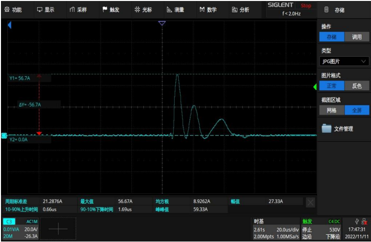
Surge curve LAG-200H-450A
