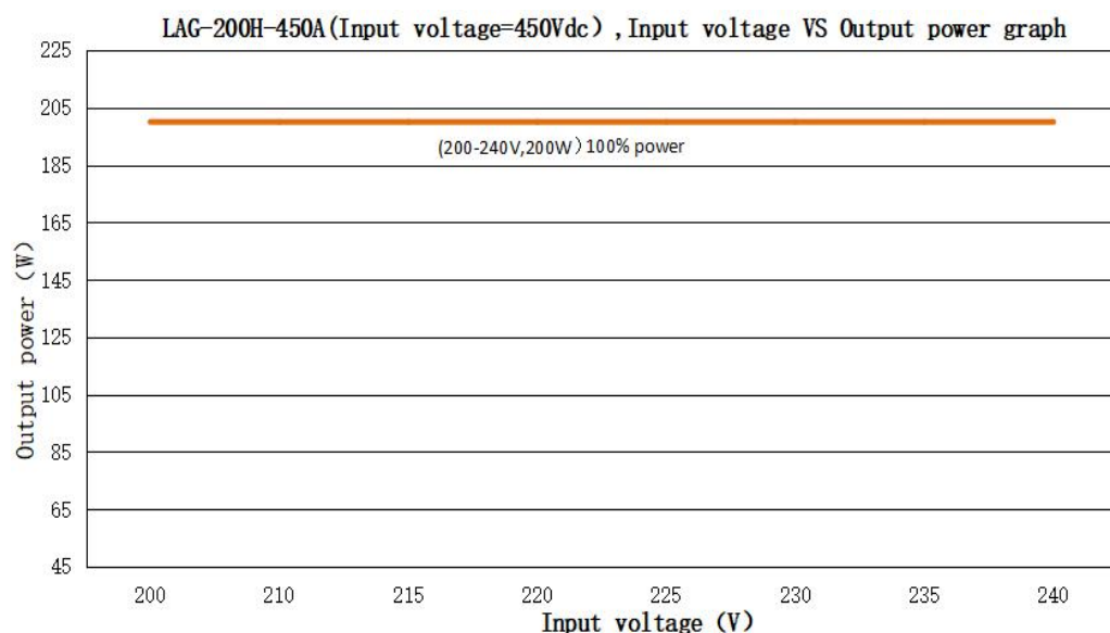
LAG-200H-450A (Vdc=450Vdc, the rated output current & power under different input voltage)
