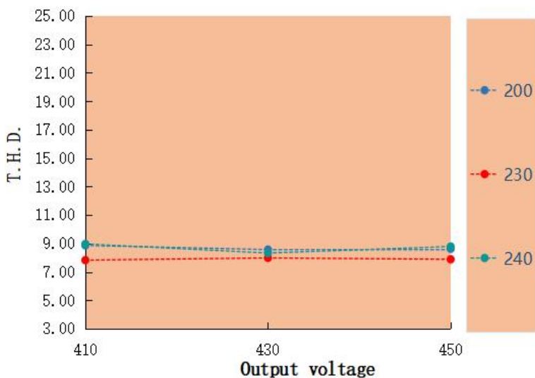
T.H.D. VS Output voltage LAG-200H-450A
