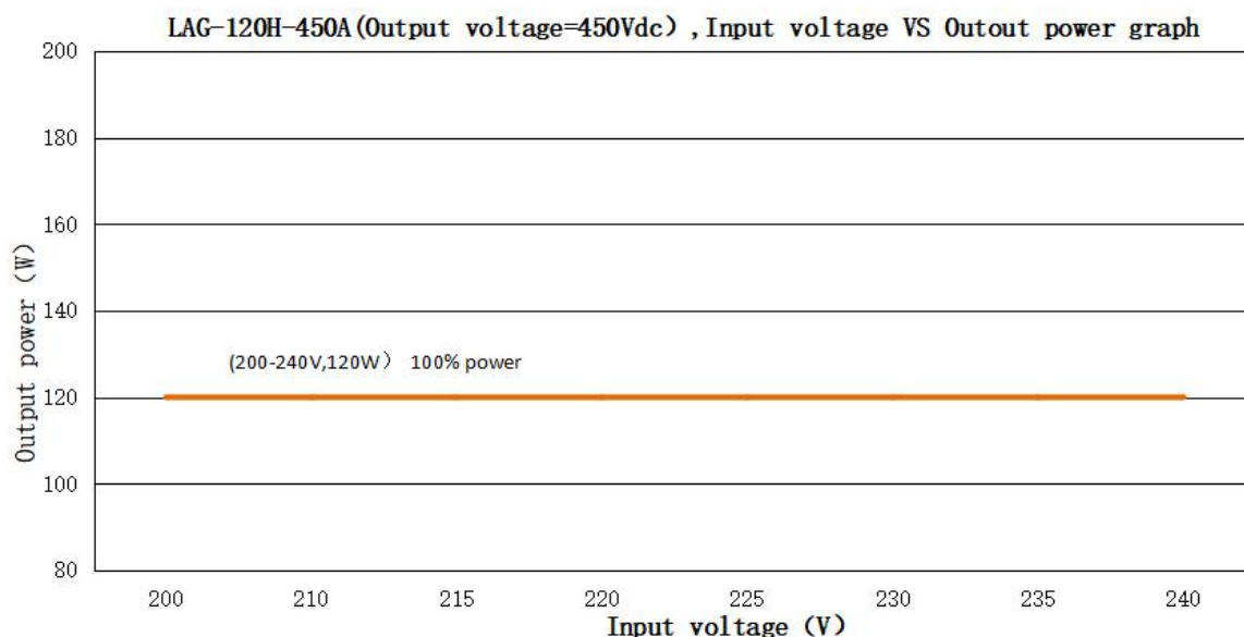
LAG-120H-450A(Vdc=470Vdc, the rated output current & power under different input voltage)
