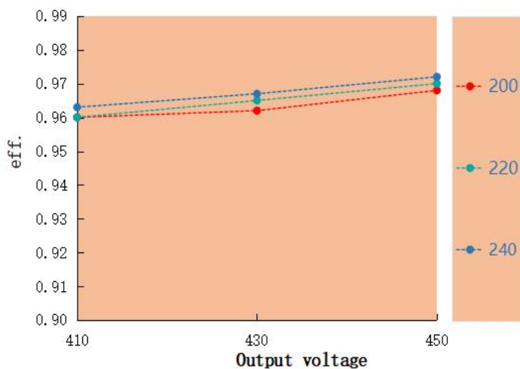
Eff. VS Output voltage LAG-120H-450A
