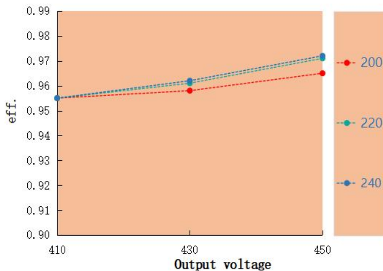
Eff. VS Output voltage LAG-120H-450A-XP
