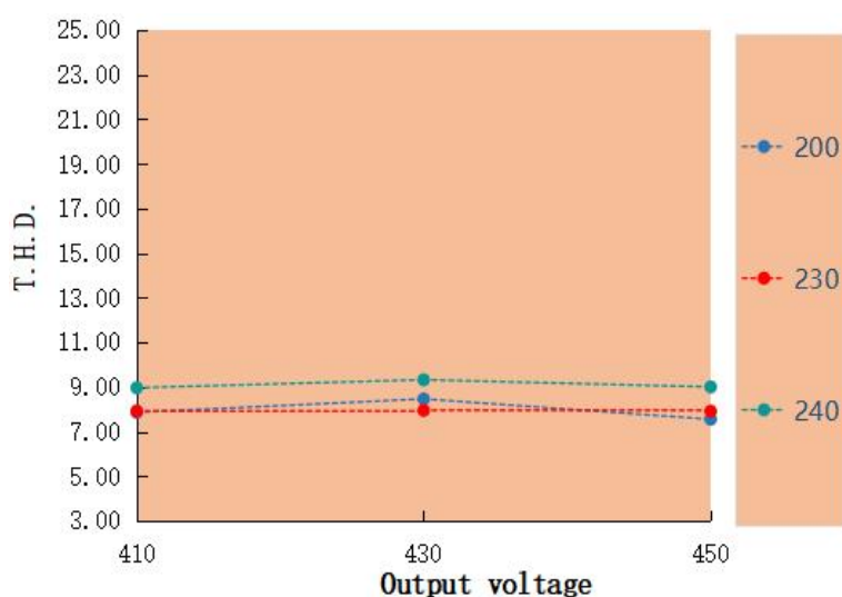
T.H.D. VS Output voltage LAG-120H-450A-XP
