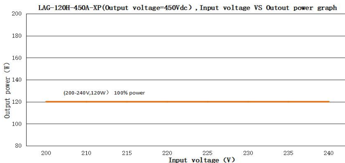
LAG-120H-450A-XP(Vdc=470Vdc, the rated output current & power under different input voltage)
