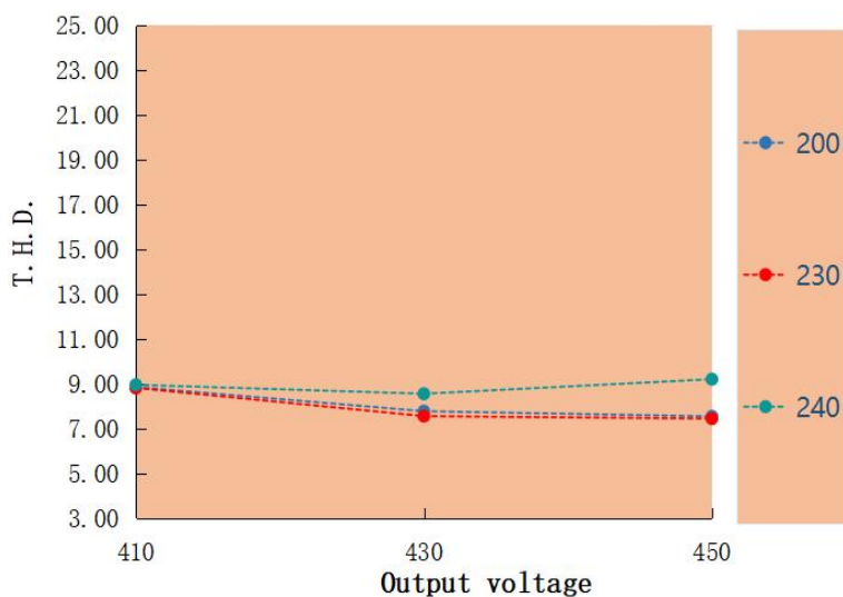
T.H.D. VS Output voltage LAG-120H-450A
