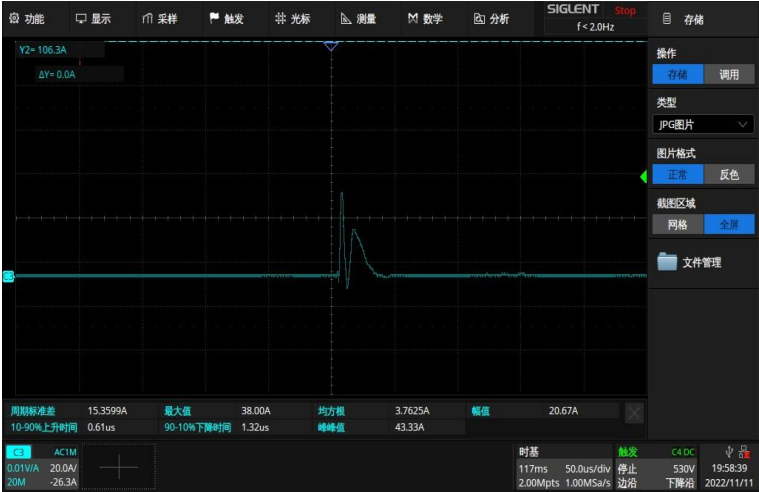
Surge curve LAG-120H-450A
