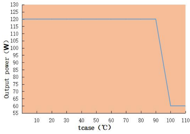
Output power VS Tcase LAG-120H-450A
