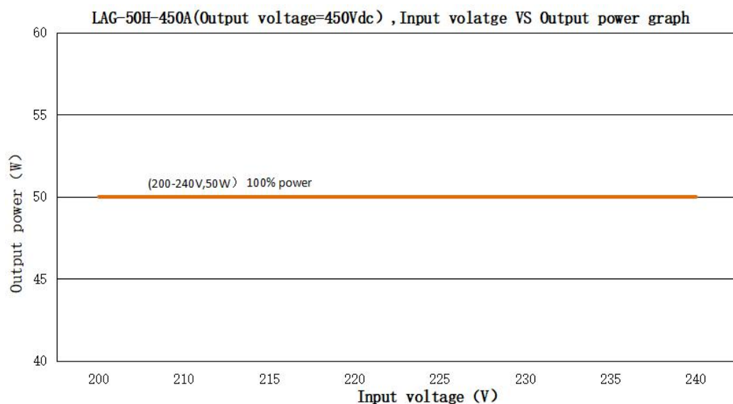
LAG-50H-450A(Vdc=470Vdc, the rated output current & power under different input voltage)
