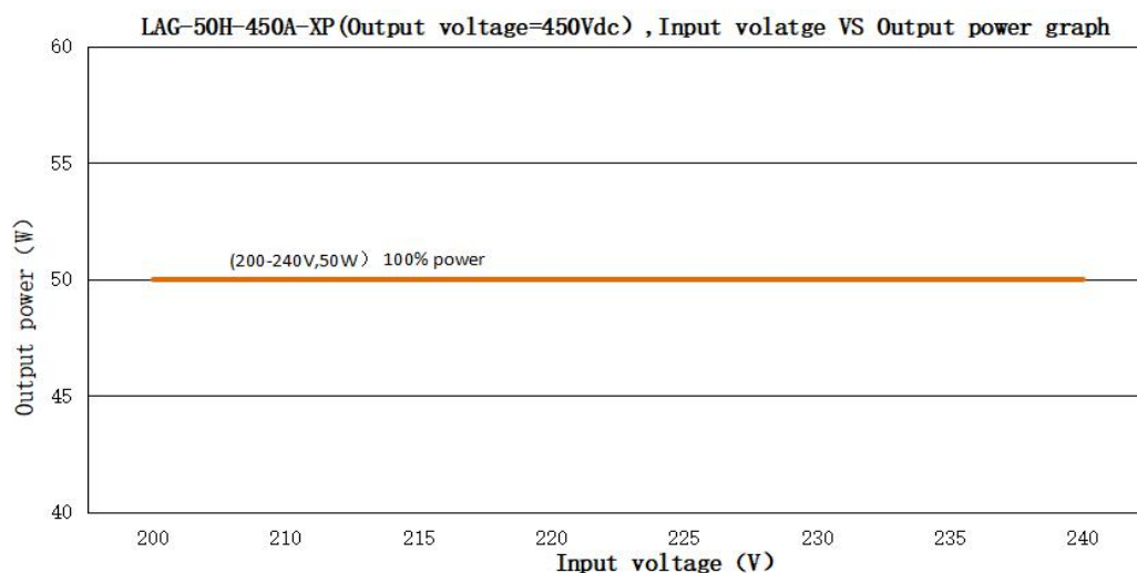
LAG-50H-450A-XP(Vdc=470Vdc, the rated output current & power under different input voltage)
