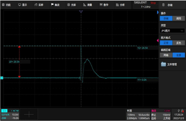
Surge curve LAG-50H-450A
