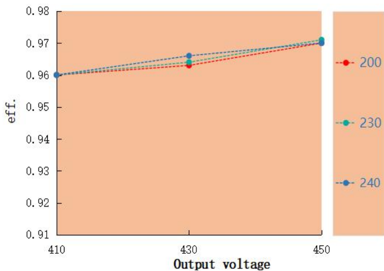
Eff. VS Output voltage LAG-50H-450A
