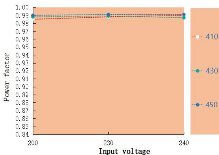
Power factor VS Input voltage LAG-50H-450A
