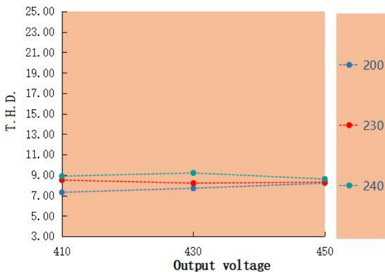
T.H.D. VS Output voltage LAG-50H-450A-XP
