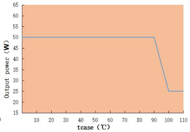
Output power VS Tcase LAG-50H-450A
