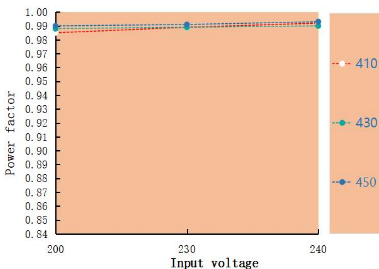
Power factor VS Input voltage LAG-50H-450A-XP
