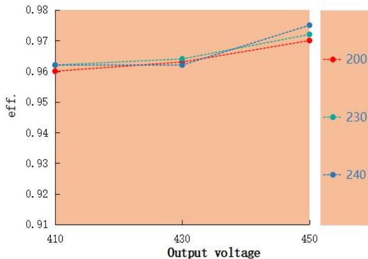
Eff. VS Output voltage LAG-50H-450A-XP
