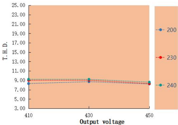
T.H.D. VS Output voltage LAG-50H-450A
