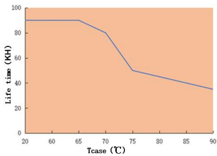
Tcase VS Life time LAG-100H-450A
