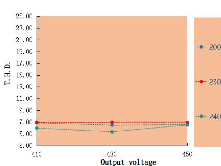
T.H.D. VS Output voltage LAG-100H-450A-XP
