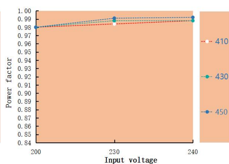
Power factor VS Input voltage LAG-100H-450A-XP
