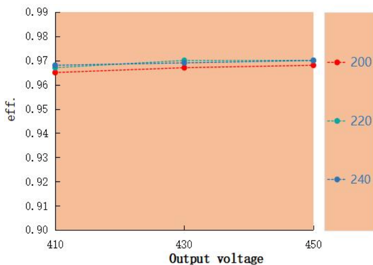
Eff. VS Output voltage LAG-100H-450A
