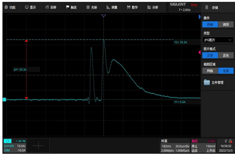
Surge curve LAG-100H-450A
