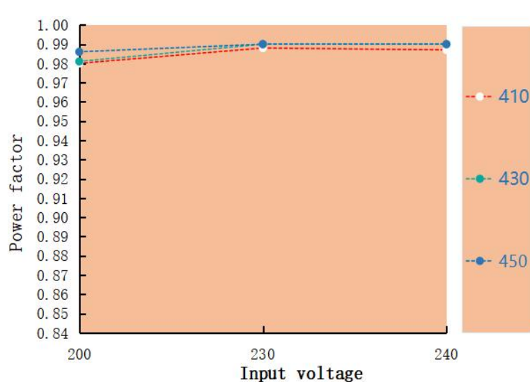
Power factor VS Input voltage LAG-100H-450A
