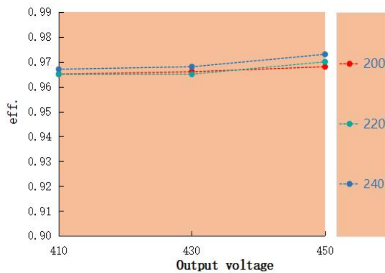
Eff. VS Output voltage LAG-100H-450A-XP
