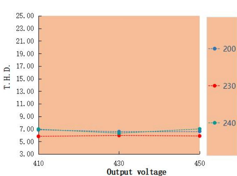
T.H.D. VS Output voltage LAG-100H-450A
