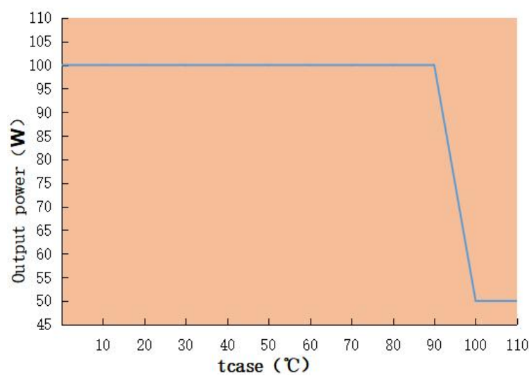
Output power VS Tcase LAG-100H-450A
