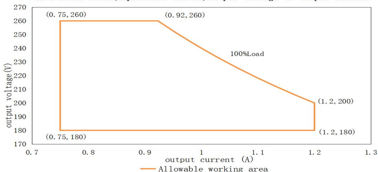
LBS-240W-260X (Import:100-277Vac) output voltage VS output current
