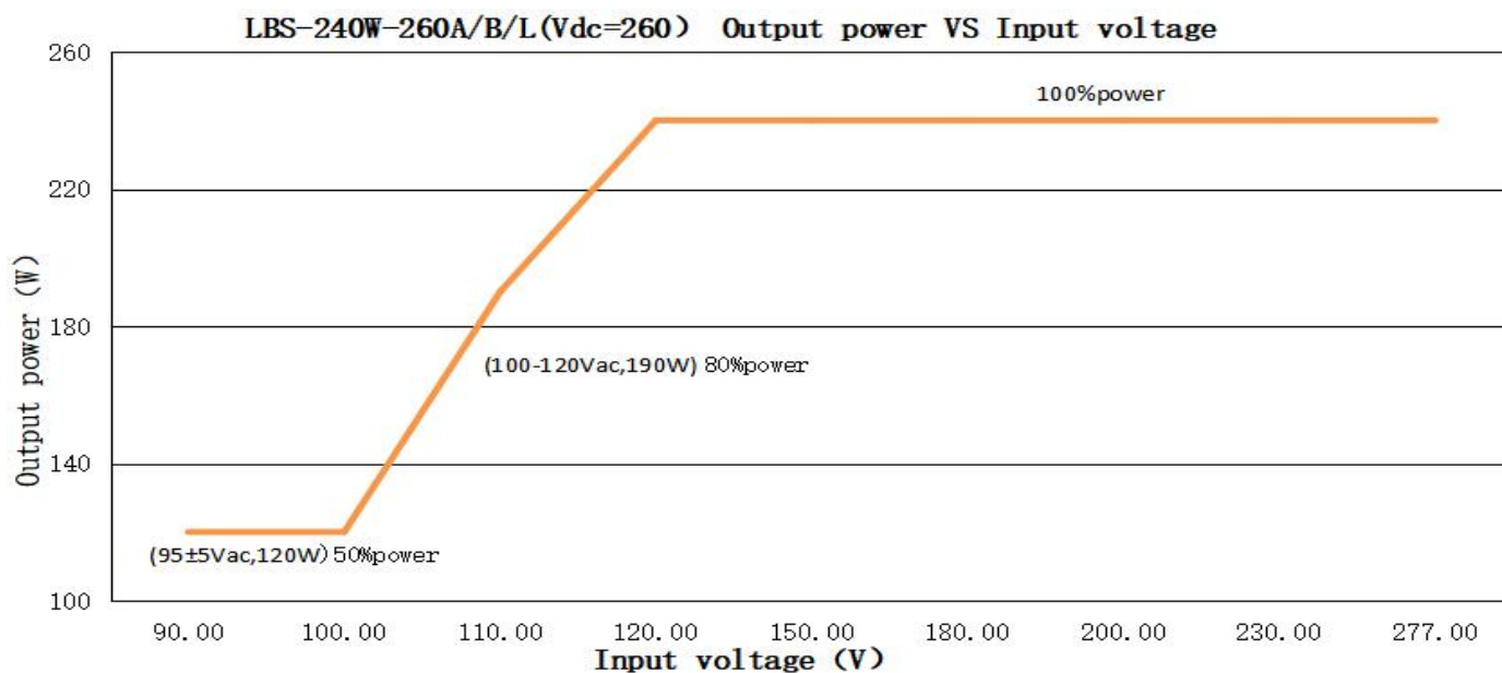
LBS-240W-260X(For output 260Vdc, the rated output current & power under different input voltage)
