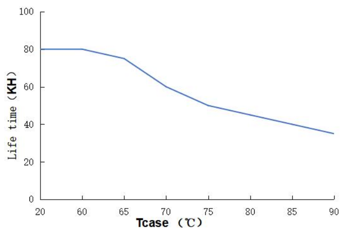
Tcse VS Life time
