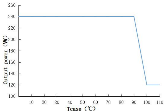
Output power VS Tcse
