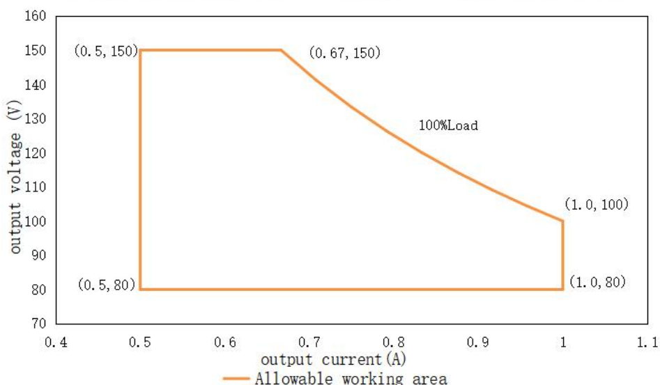
LBS-100W-150A/P/L(input:120-277Vac)output voltage VS Output current
