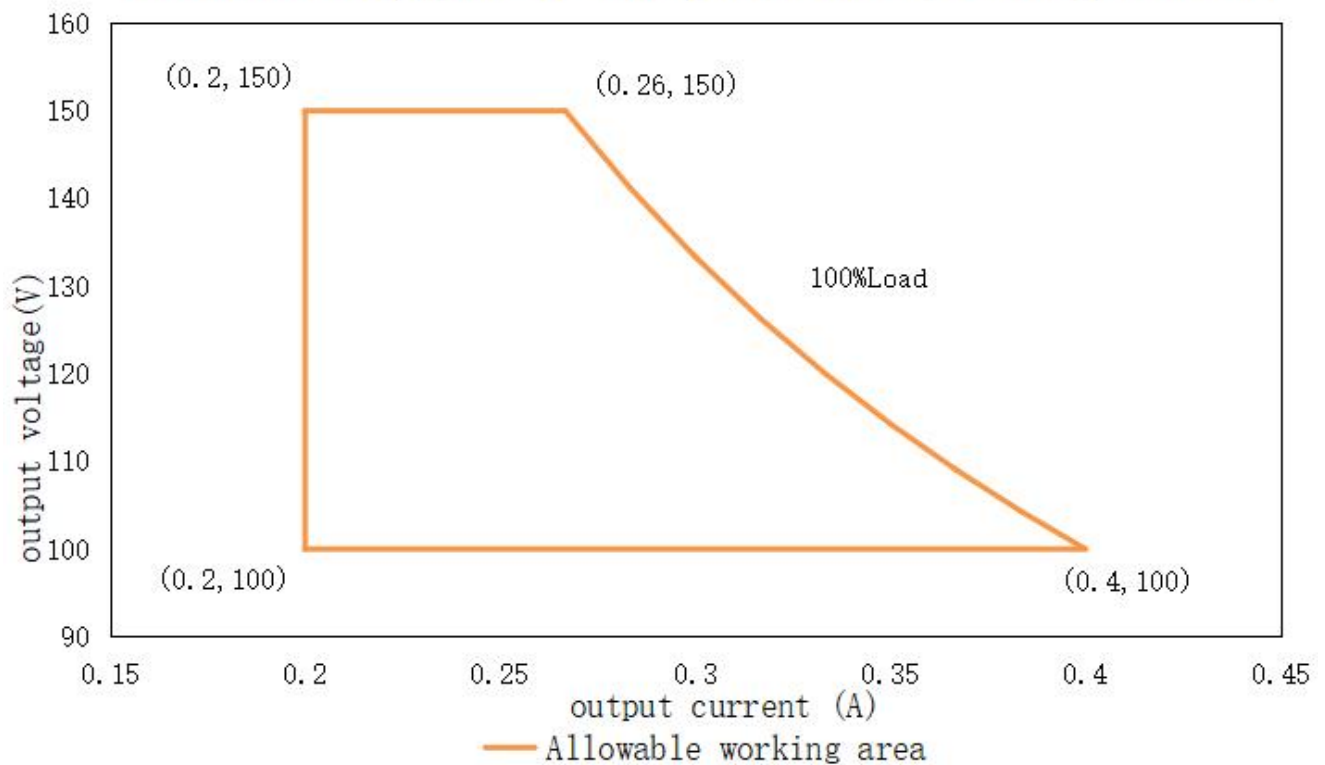
HBG-40D-150X (Import: 320-480Vdc) output voltage VS output current
