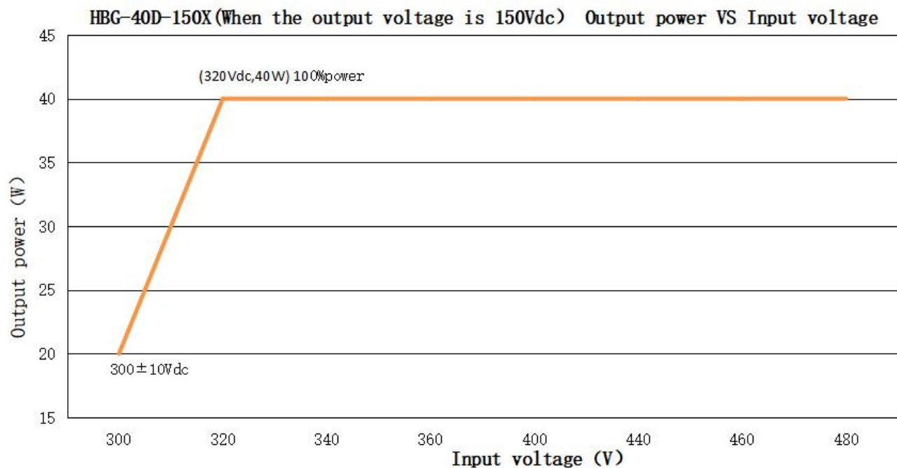
HBG-40D-150X (Rated output current value and output power corresponding to different input voltages when the output voltage is 150Vdc)
